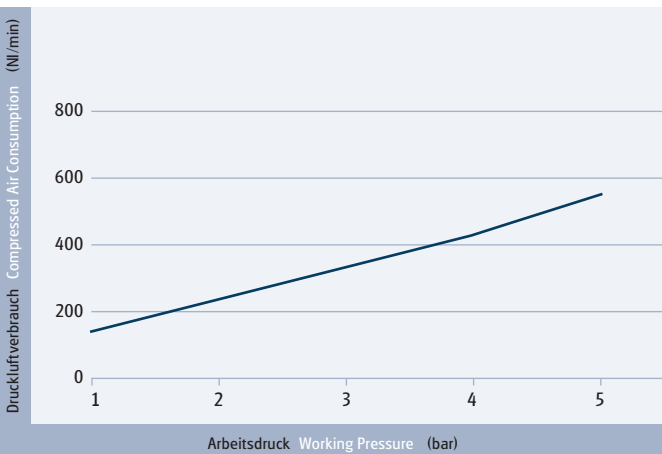
Druckluftverbrauch Air Consumption
